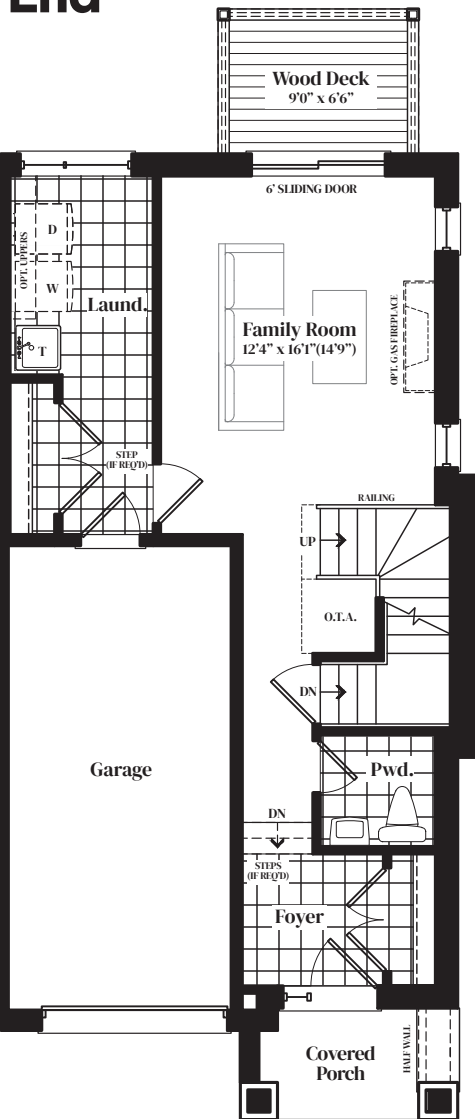
LOWER LEVEL Elev. A Corner
