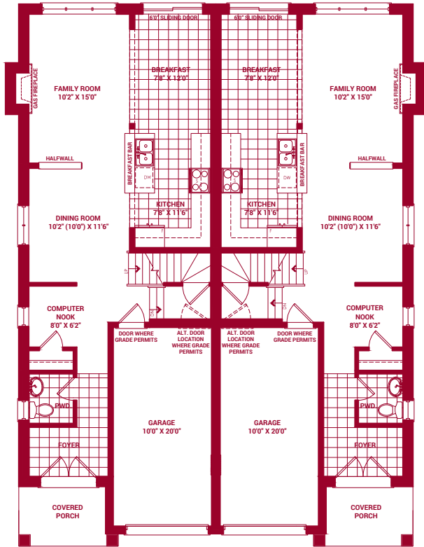
Elevation A Ground Floor
