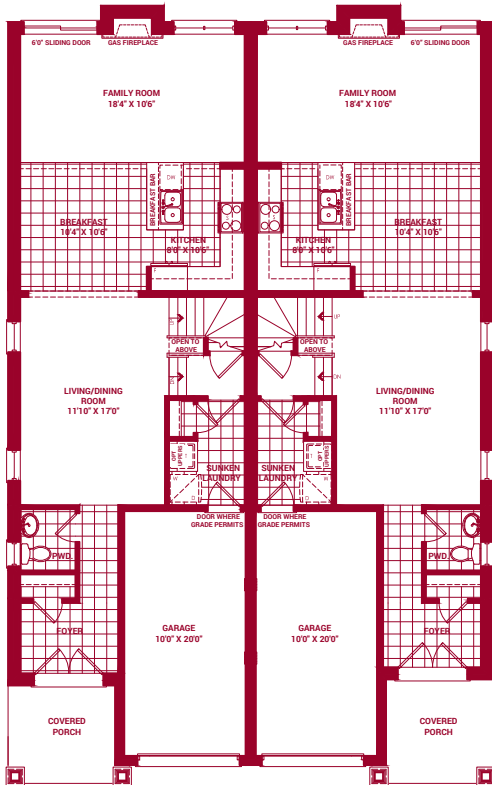
Elevation A Ground Floor
